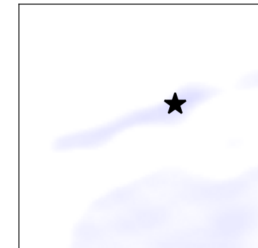
Deterministic prediction
